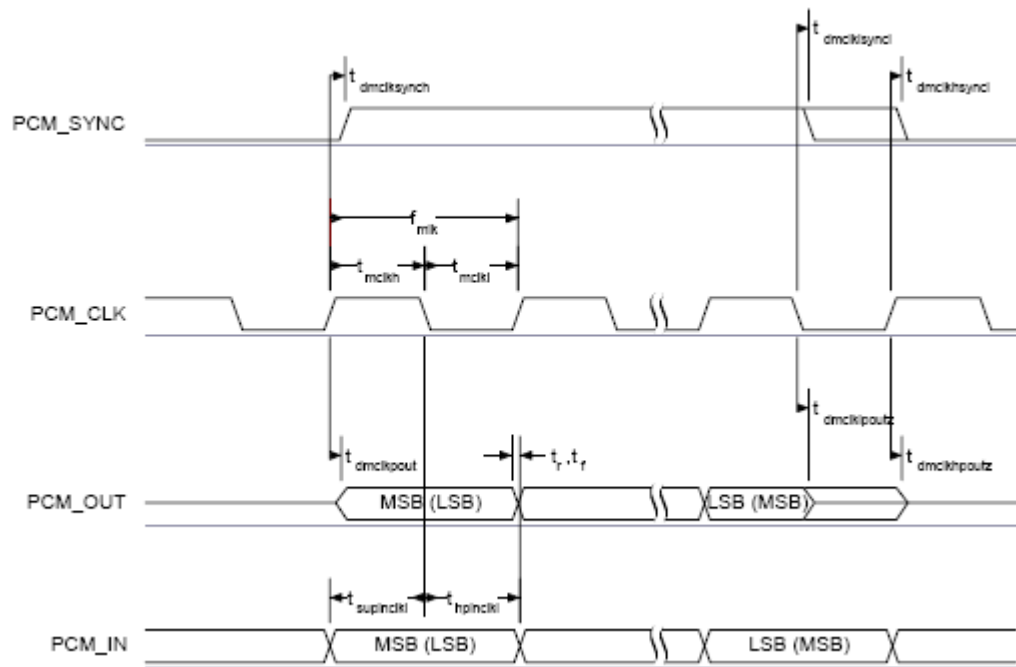
Figure 13: PCM Master Timing Long Frame Sync
