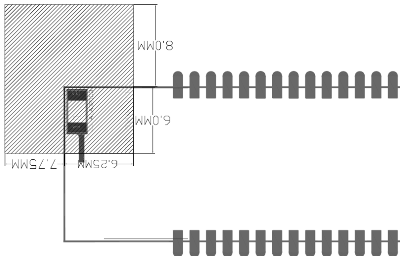
Figure 20: Clearance area of antenna
