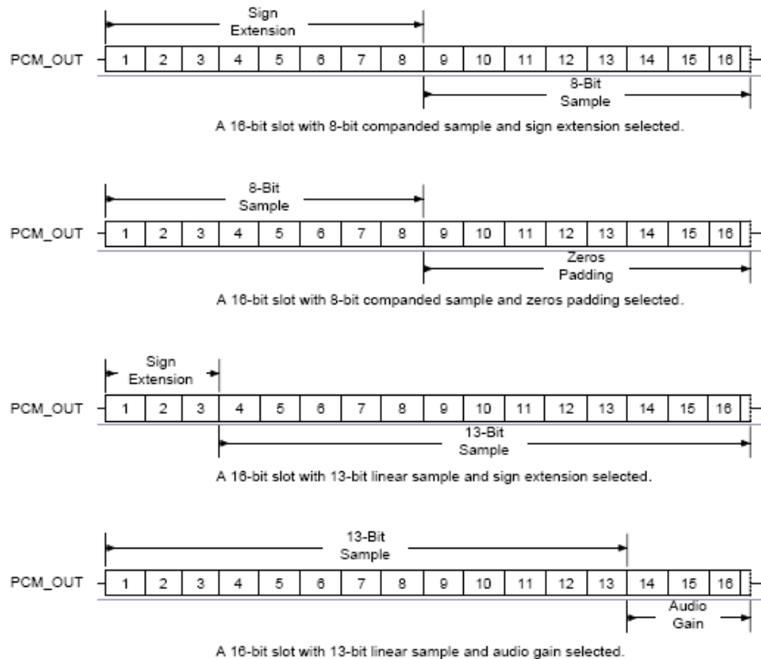
Figure 12: 16-Bit Slot Length and Sample Formats
