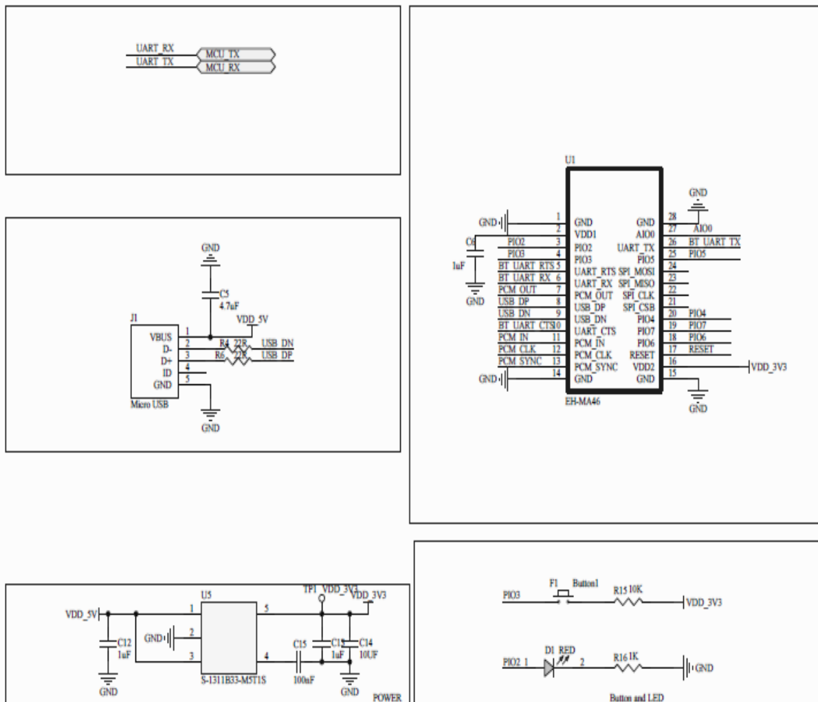
Figure 18: Reference Design
