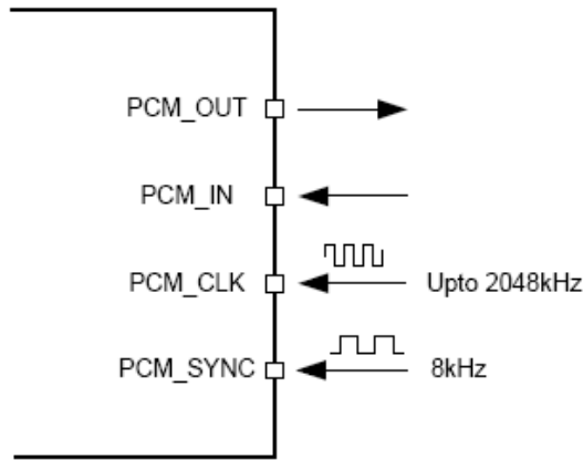
Figure 7: Configured PCM as a Slave
