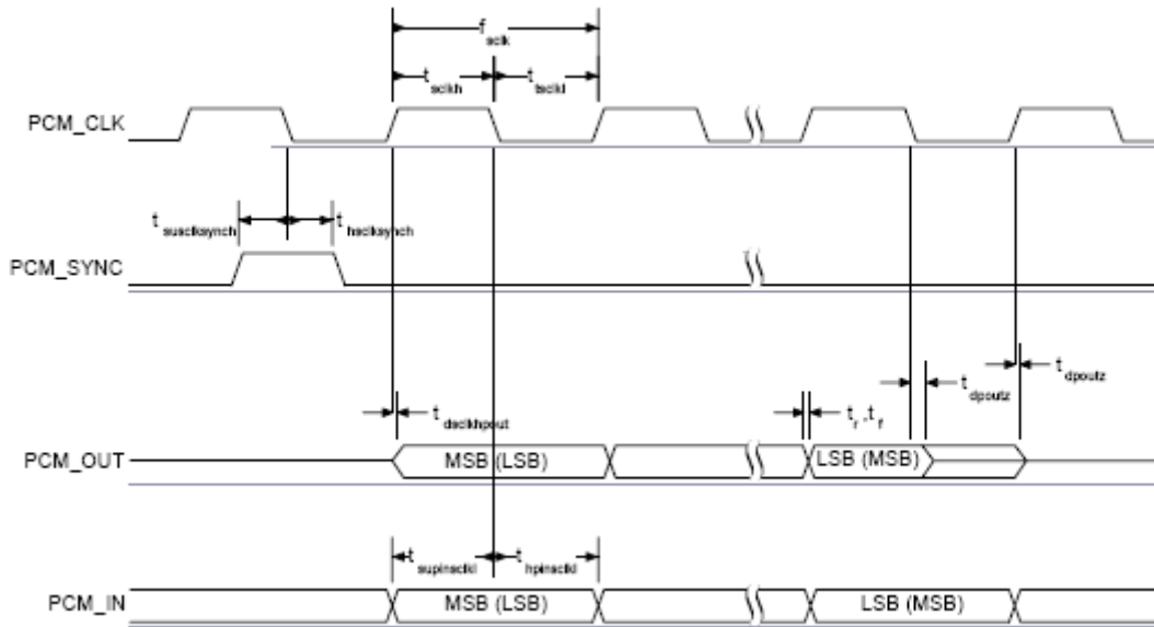
Figure 16: PCM Slave Timing Short Frame Sync
