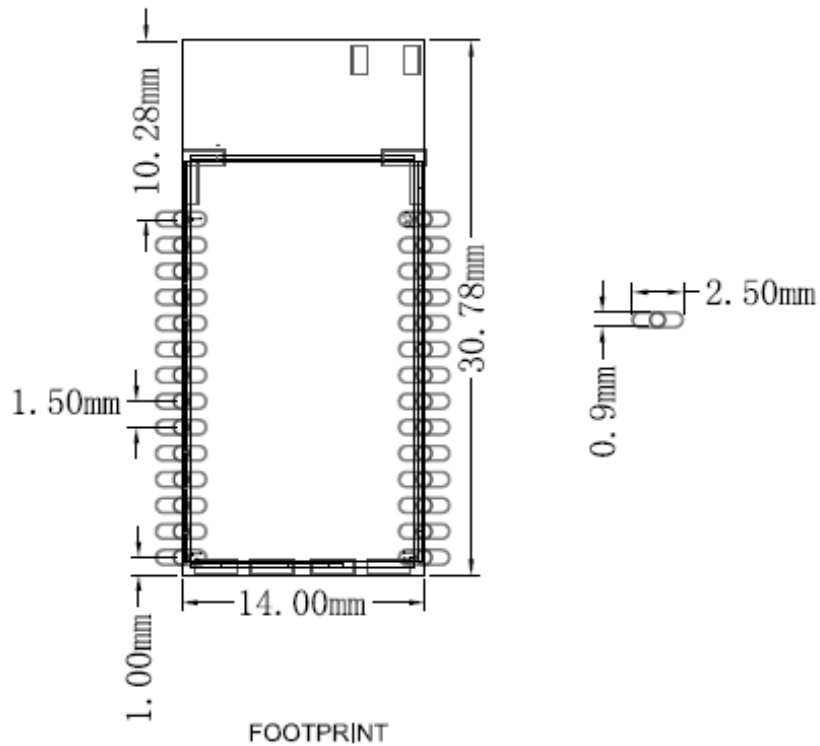
Figure 19: Recommended PCB Mounting Pattern (Unit: mm, Deviation:0.02mm)TOP View
