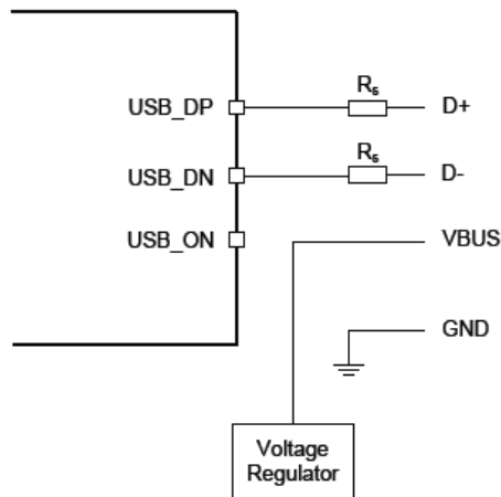
Figure 17: USB Connections
