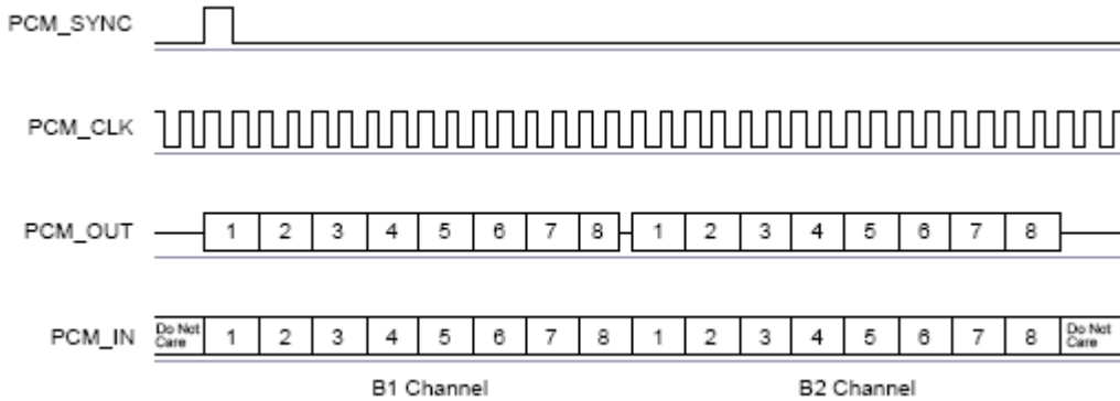
Figure 11: GCI Interface
