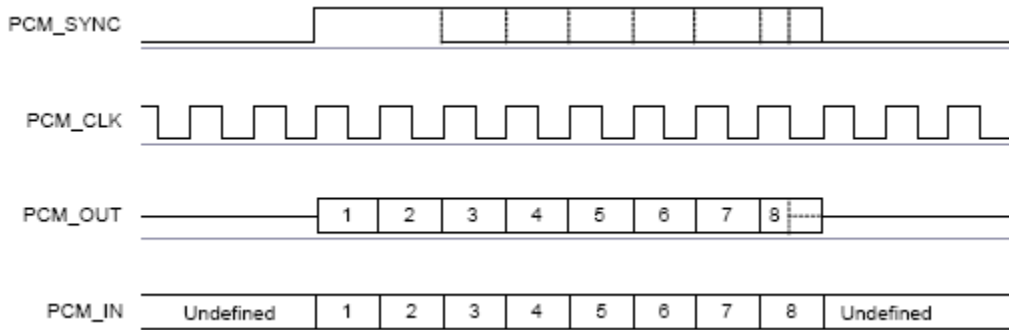
Figure 8: Long Frame Sync (Shown with 8-bit Companded Sample)
