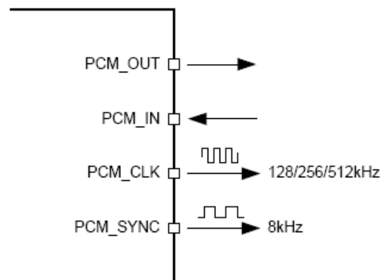
Figure 6: Configured PCM as a Master
