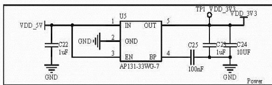
Figure 16: Reference Design
