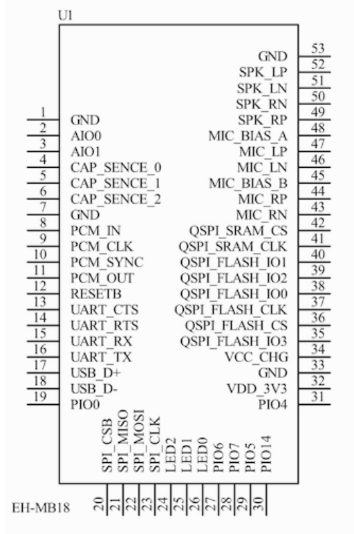
Figure 1: Pinout of EH-MB18
