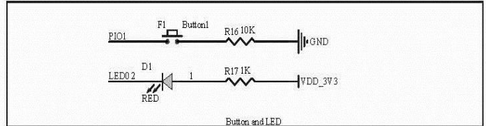
Figure 16: Reference Design
