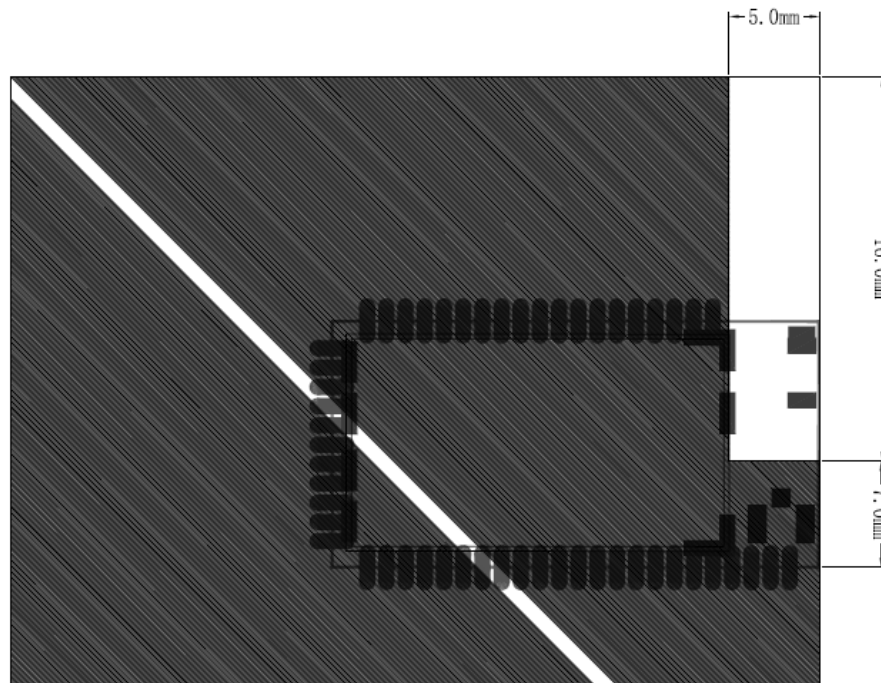
Figure 18: Clearance Area of Antenna
